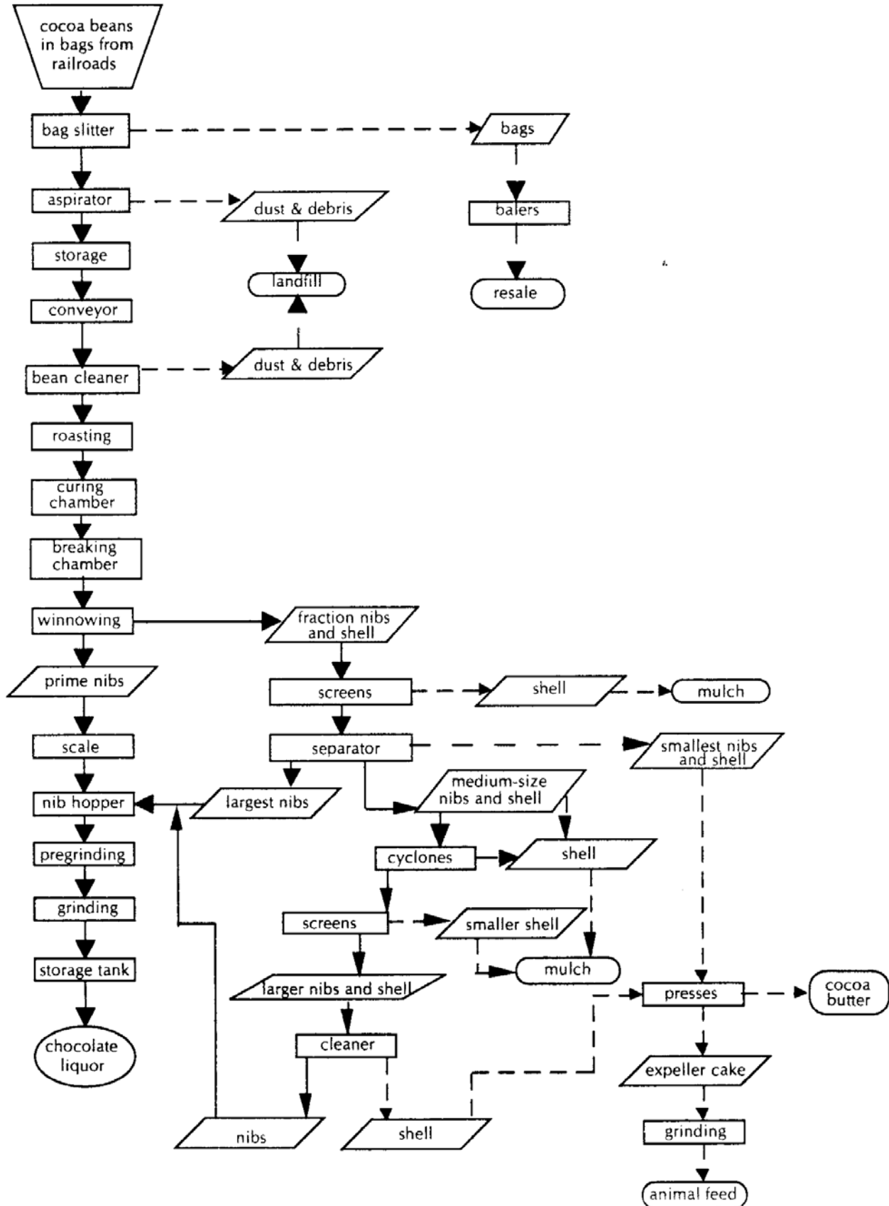
Figure 16.1 Flowchart of cocoa bean processing related FPRs
