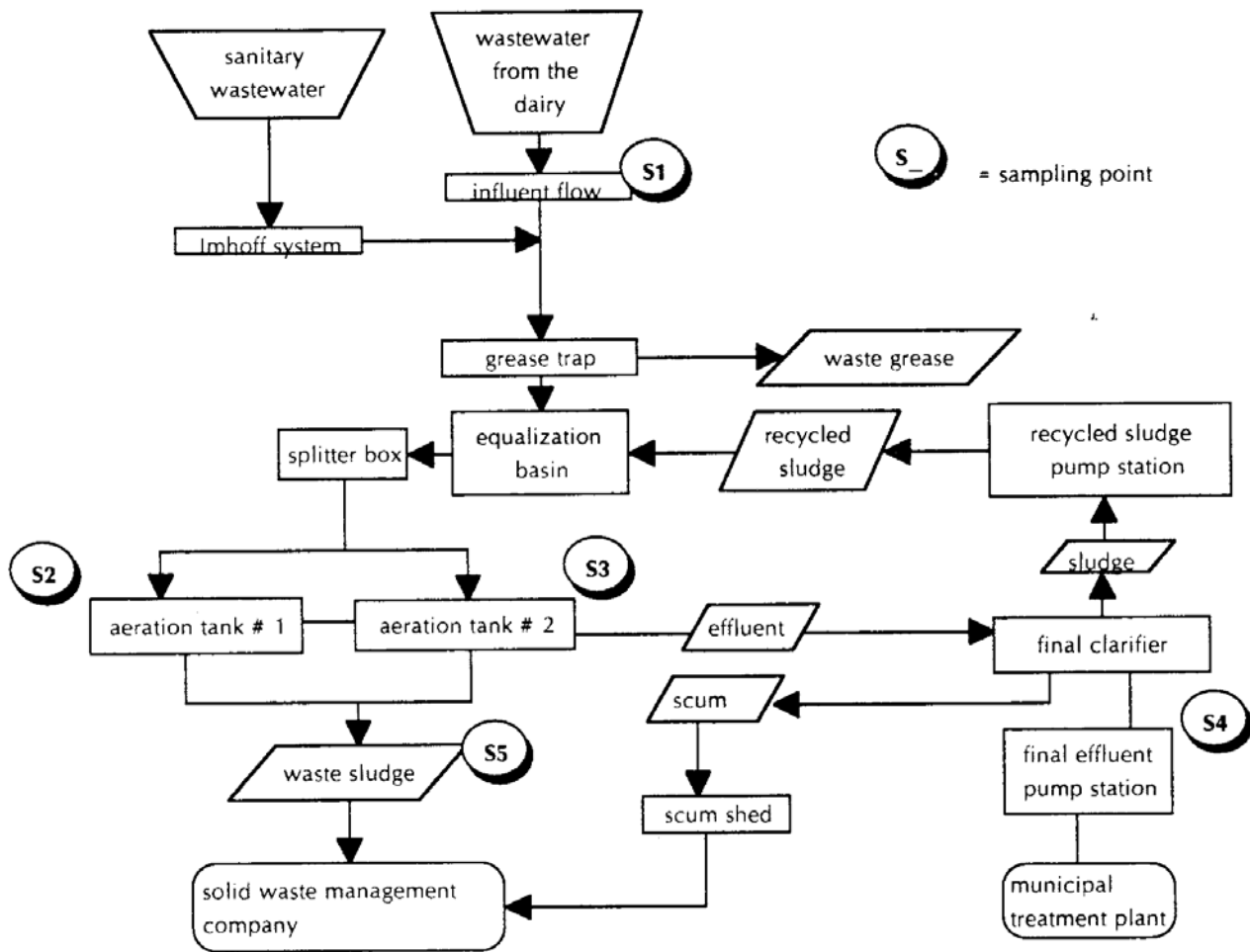
Figure 15.1 Flowchart of a wastewater treatment plant at a dairy processing facility
