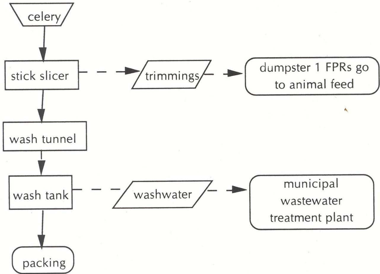
Figure 12.7 Celery process line
