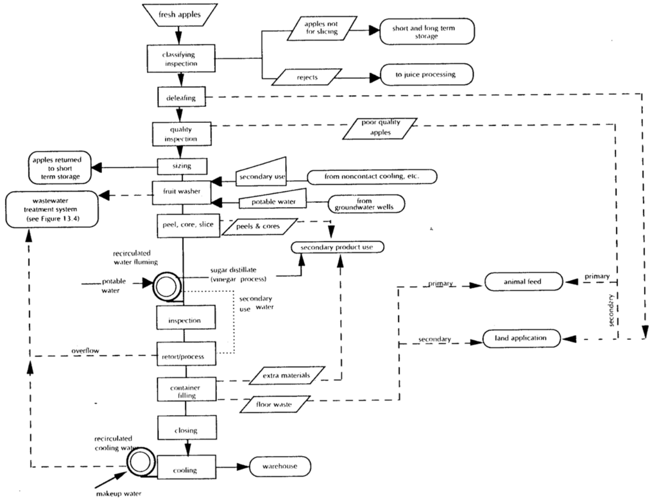
Figure 13.3 Flowchart of apple slice processing
