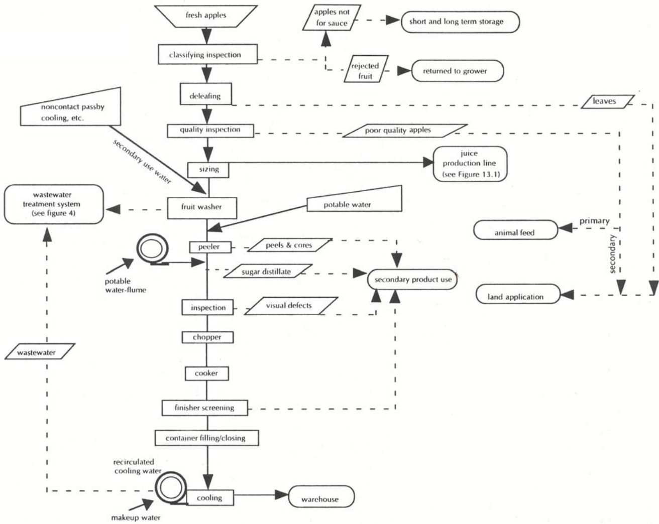
Figure 13.2 Flowchart of apple sauce processing
