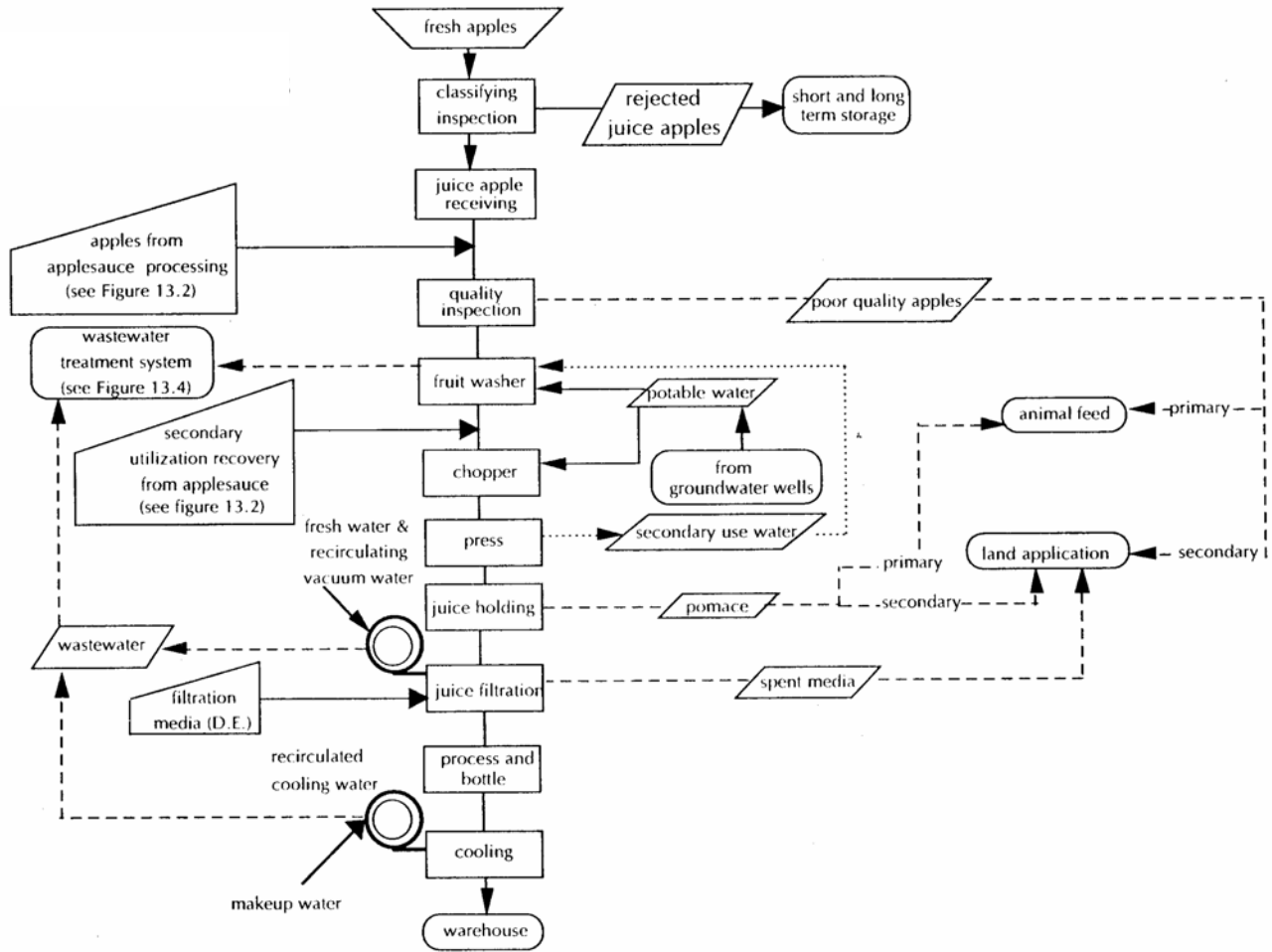
Figure 13.1 Flowchart of apple juice processing
