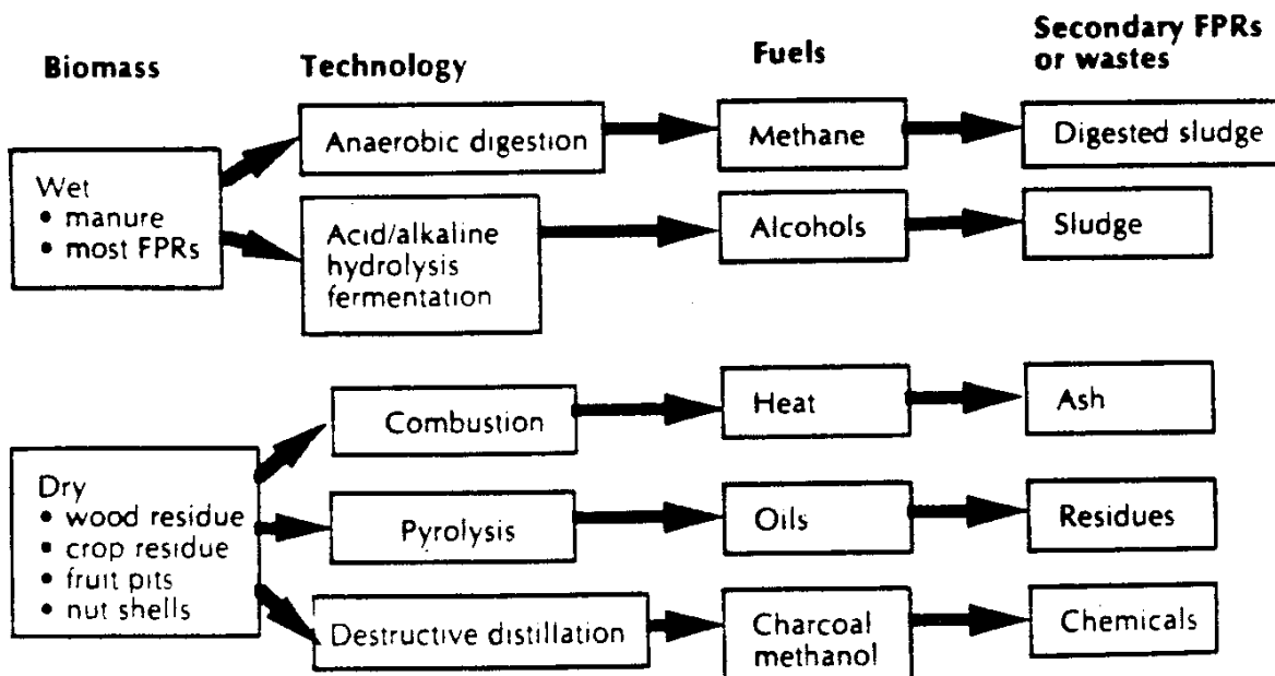
Figure 6.1 Possibilities of producing fuel form FPRs
