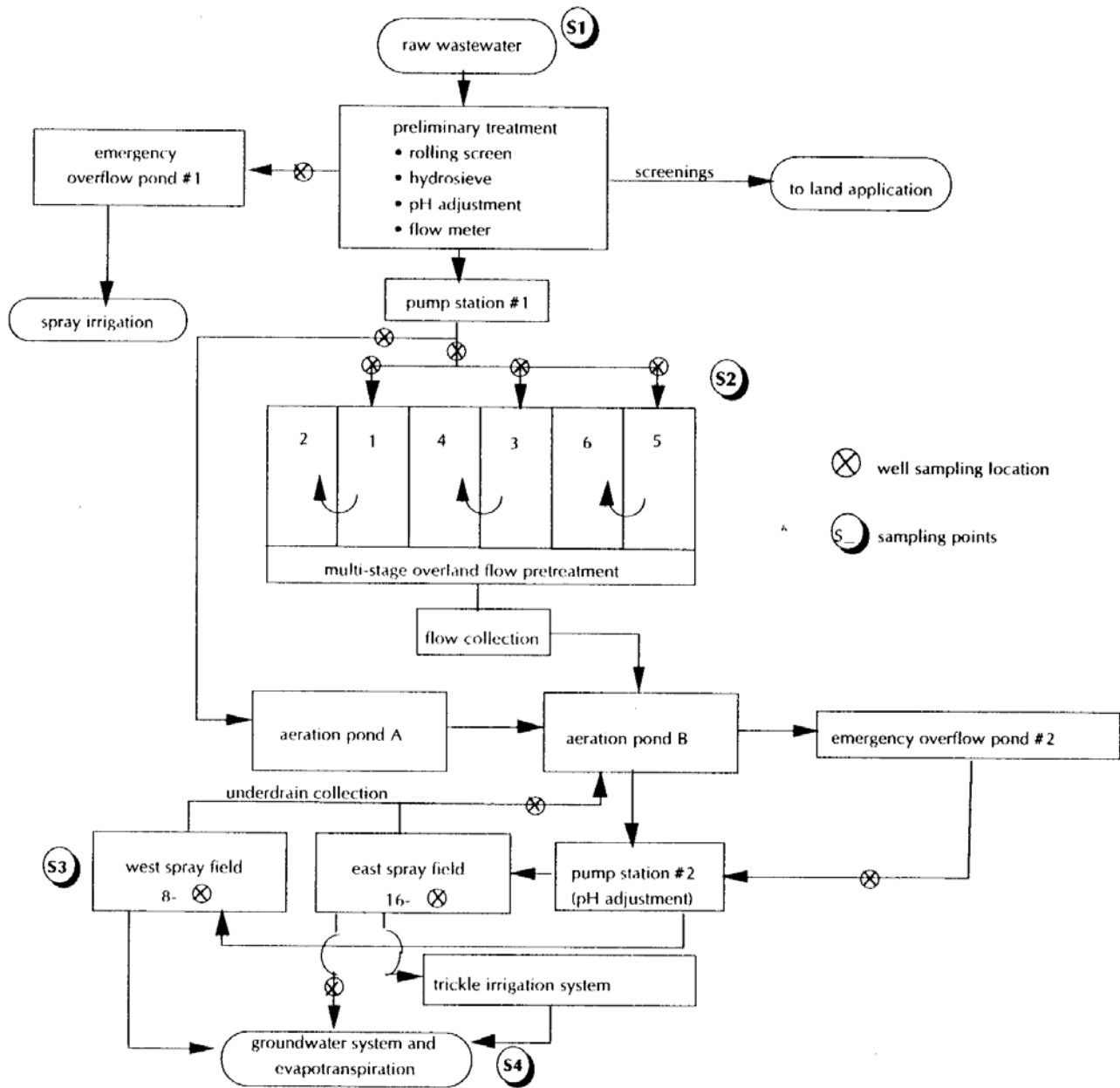
Figure 13.4 Flowchart for wastewater treatment and disposal at a fruit processing plant
