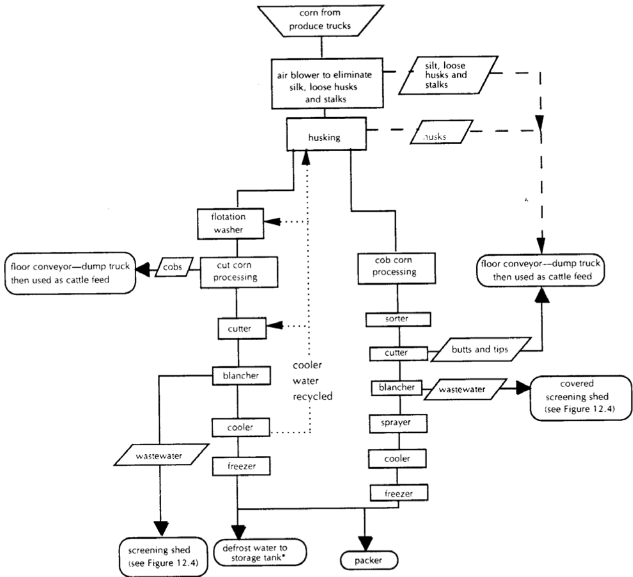
Figure 12.1 Flowchart of cob/cut corn processing and related FPRs
