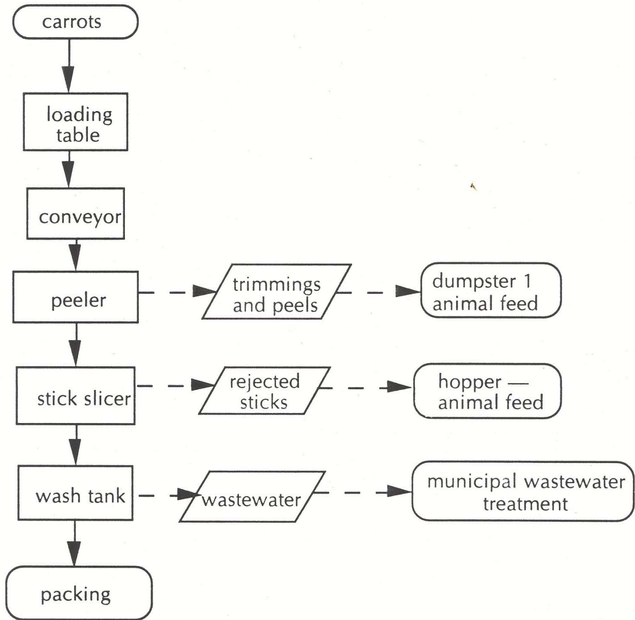
Figure 12.6 Carrot process line
