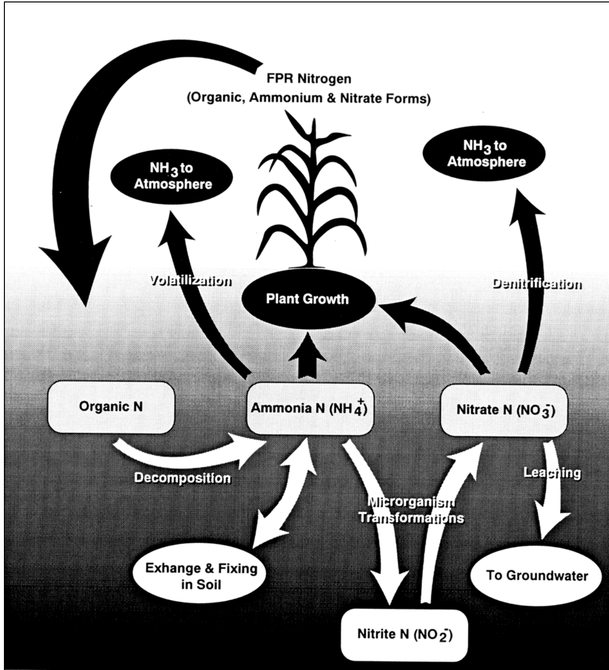
Figure 8.2 FPR nitrogen transformations and potential fates in a land application system
