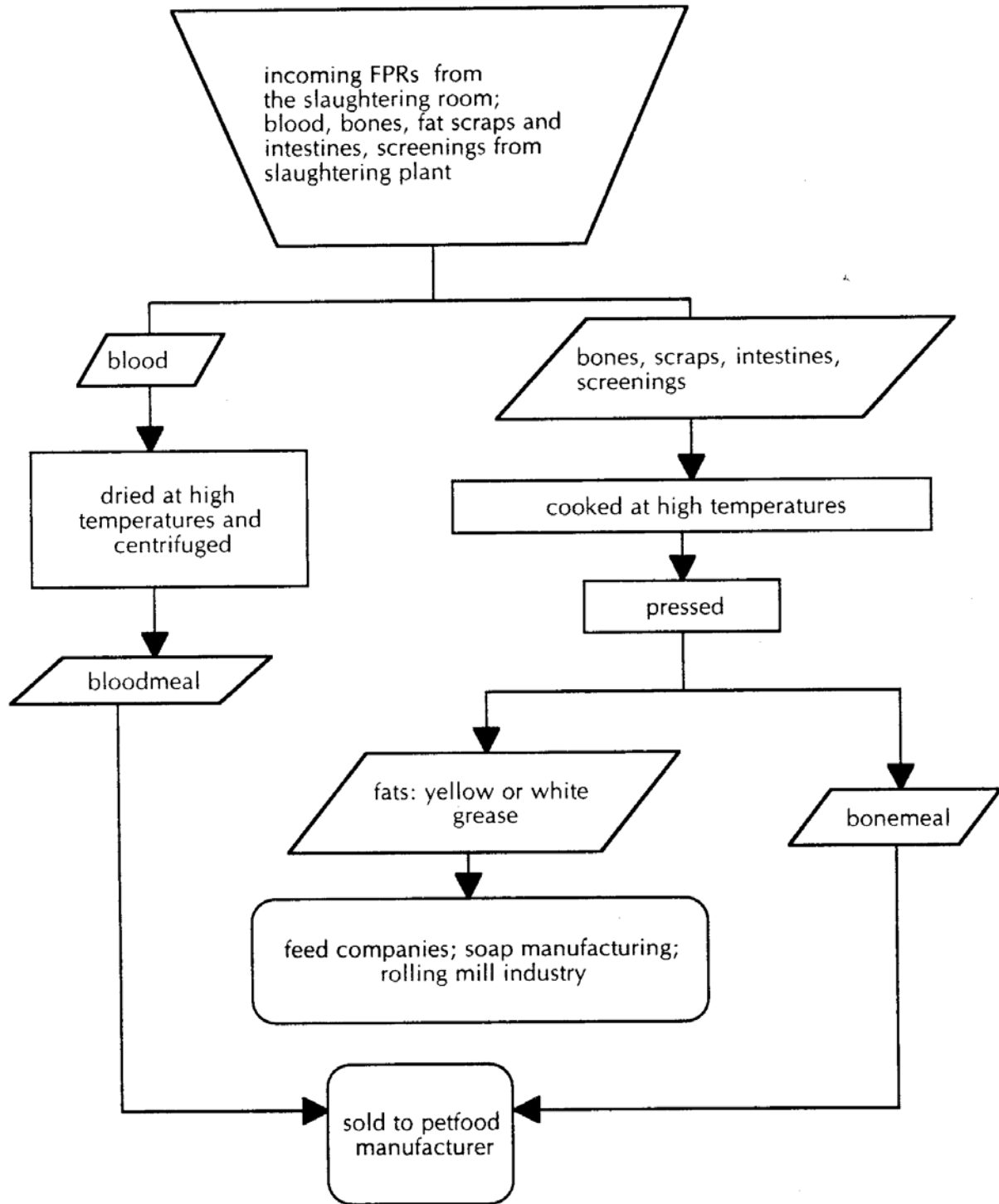
Figure 14.3 FPR flows for a rendering operation at a pork processing facility
