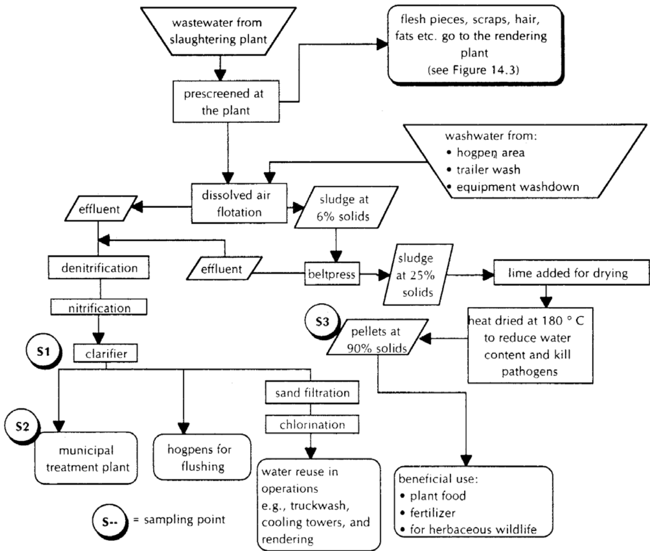
Figure 14.2 Wastewater treatment at a pork processing facility
