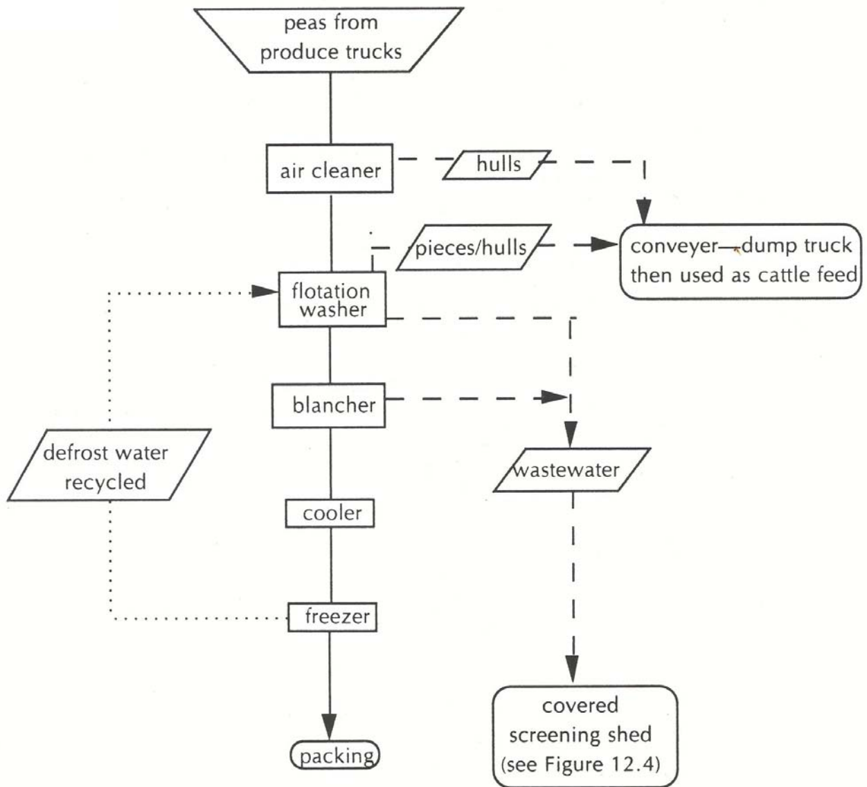
Figure 12.3 Flowchart of pea processing and related FPRs
