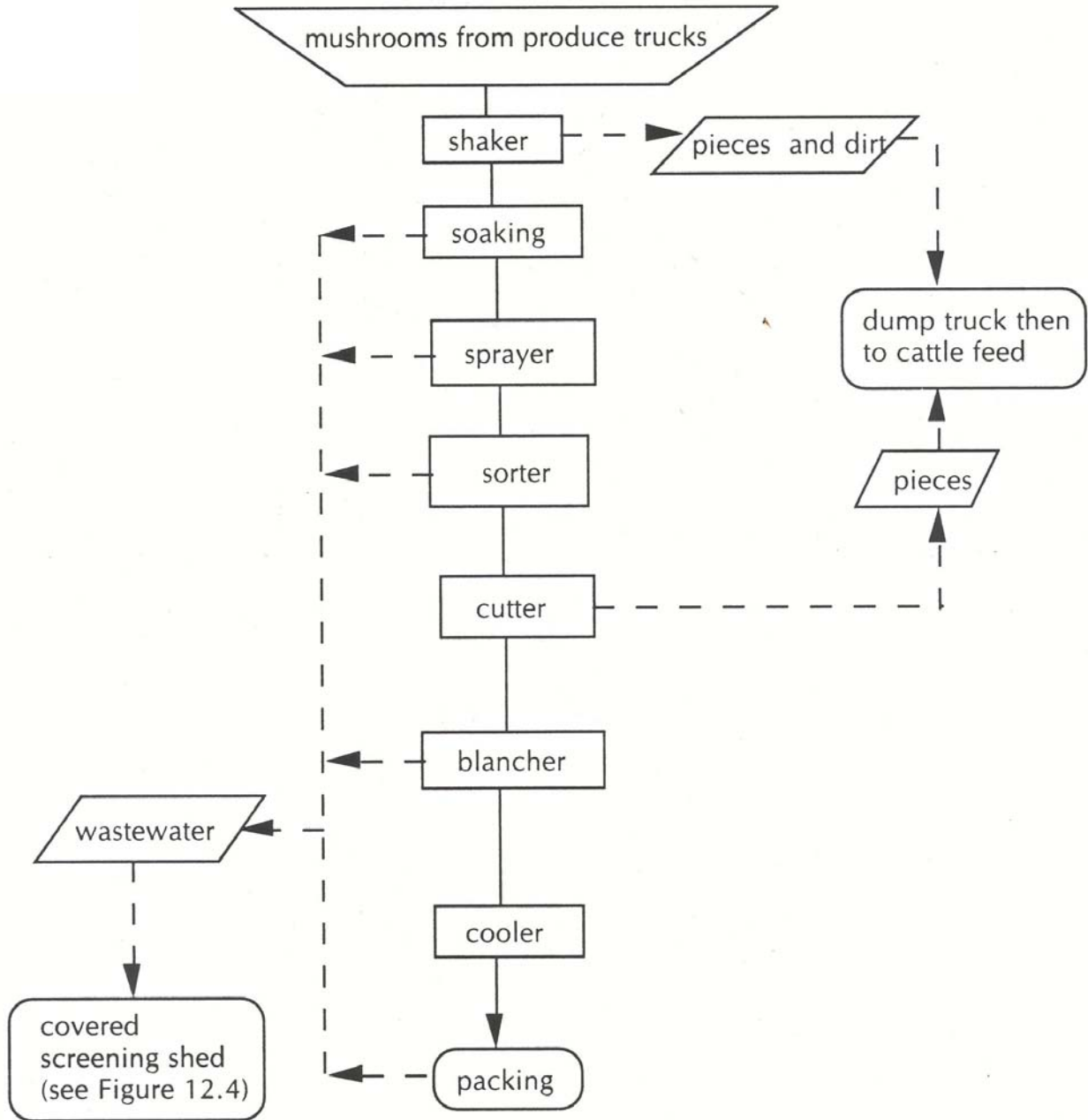
Figure 12.2 Flowchart of mushroom processing and related FPRs
