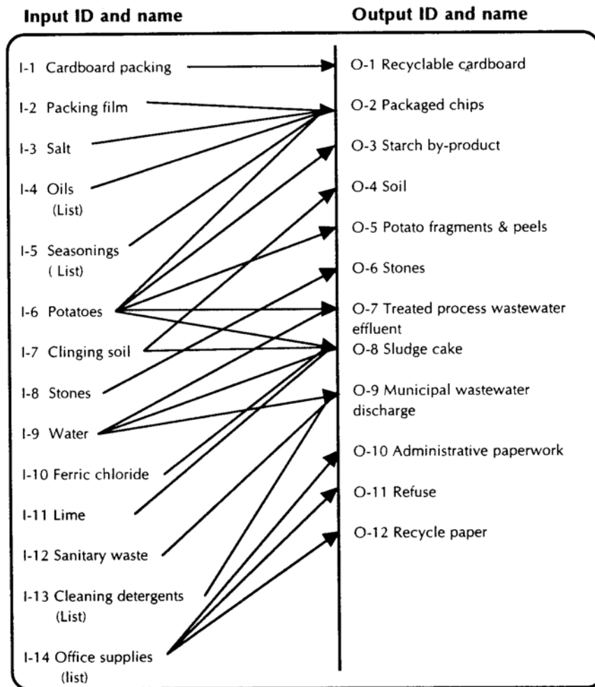
Figure 1.1: Connecting FPR inputs and outputs for a potato chip processor
