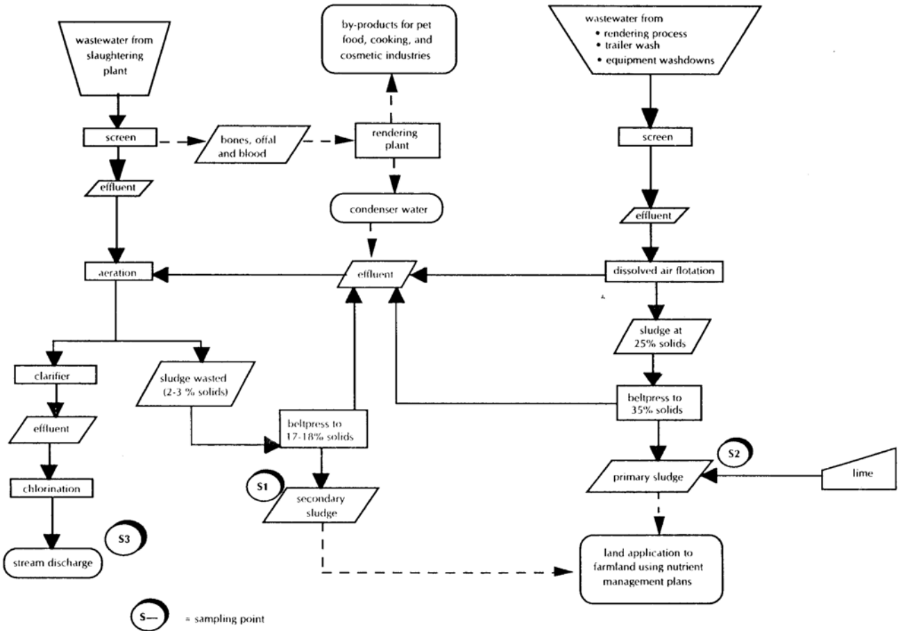
Figure 14.1 FPR flowchart for wastewater treatment processes at a meat processing and rendering facility
