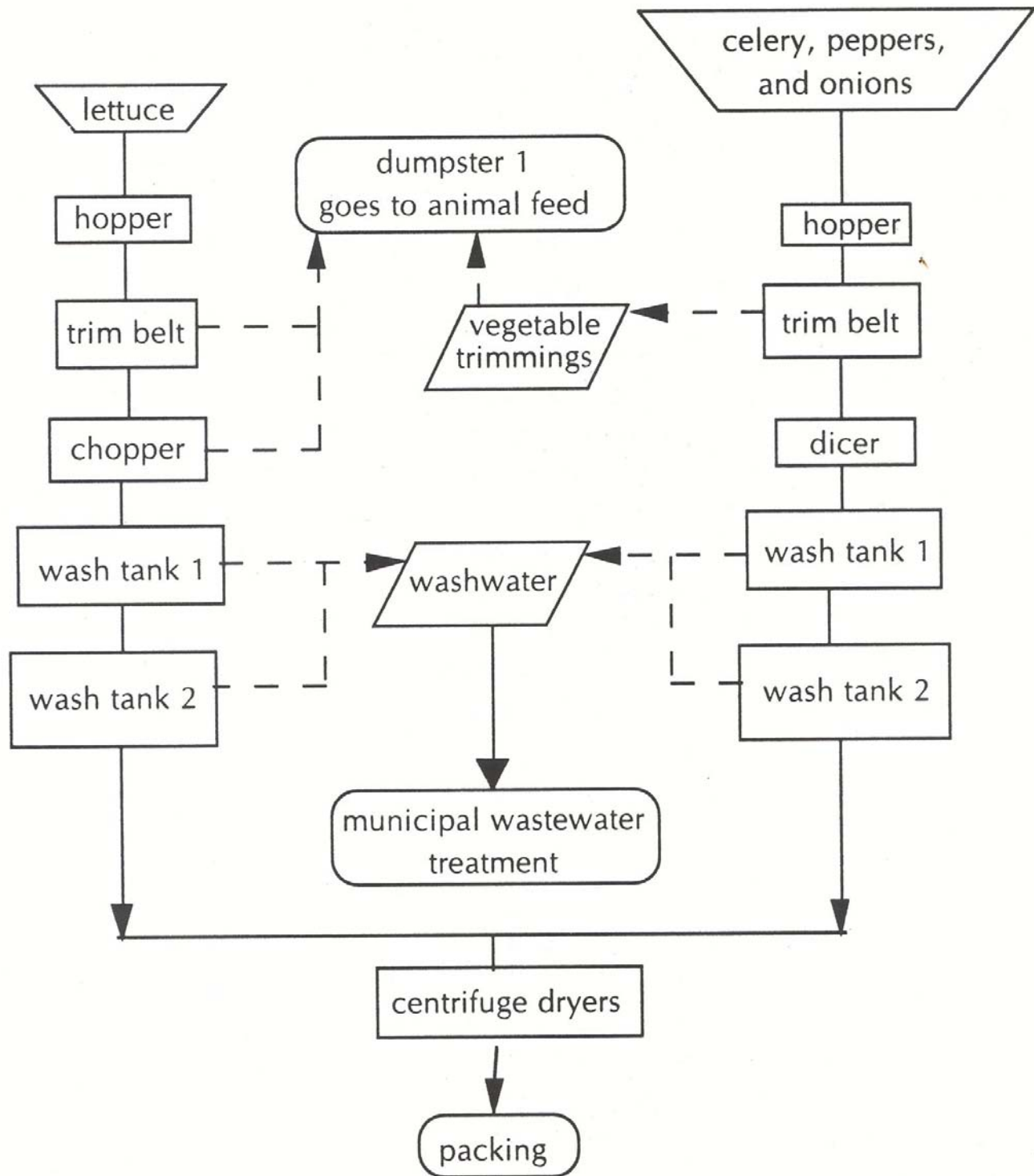
Figure 12.5 Process lines for lettuce, celery, peppers, and onions
