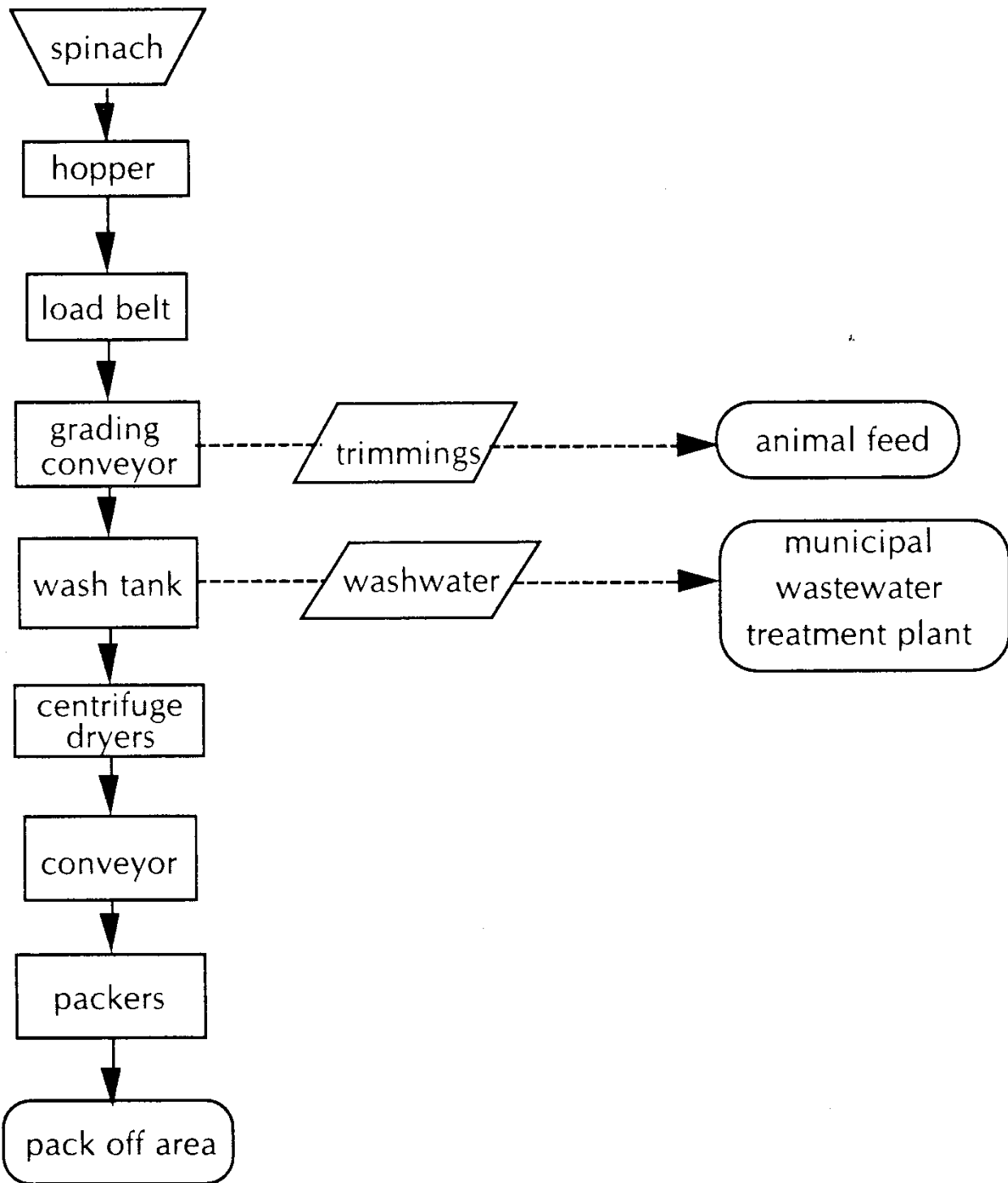
Figure 12.10 Spinach process line
