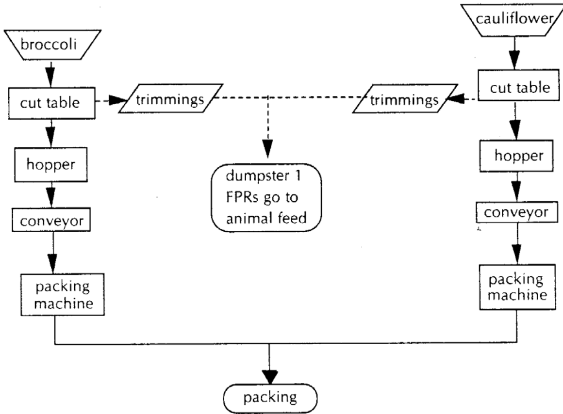
Figure 12.8 Broccoli and cauliflower process line
